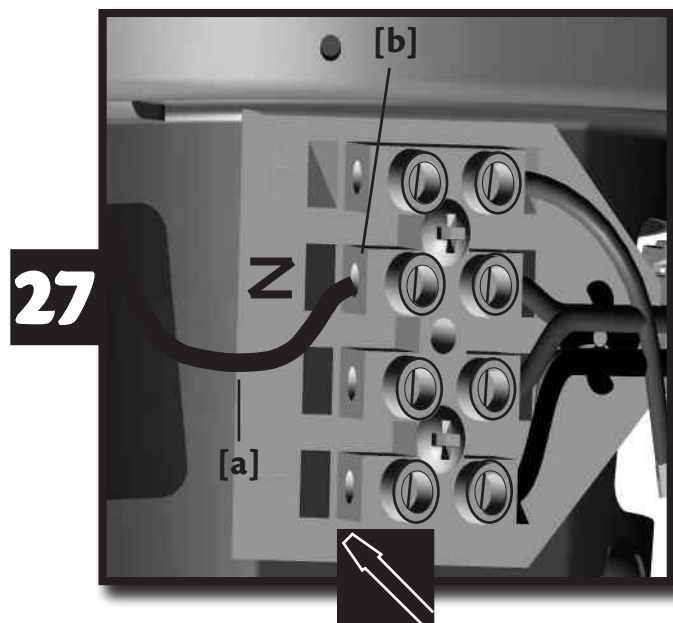
Neutral wire [a] (blue) to terminal [b] marked "N".
